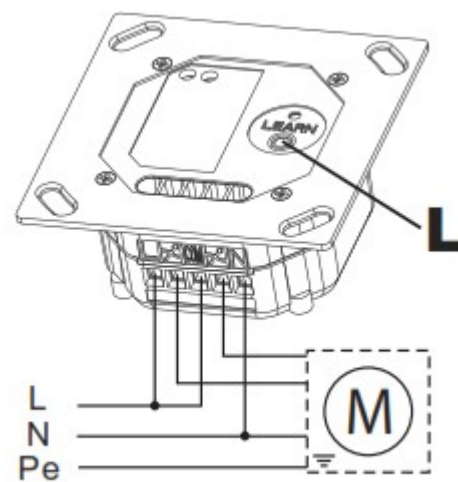
Intertechno ITL 500
